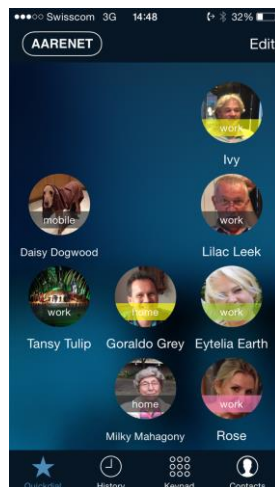
QUICKDIAL KEYS
