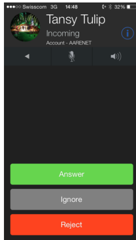
INCOMING CALL
