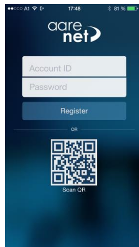
USER REGISTRATION
