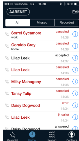
CALL HISTORY
