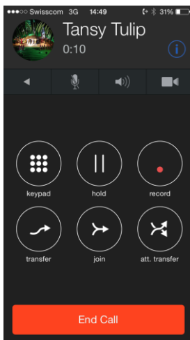
ACTIVE CALL
